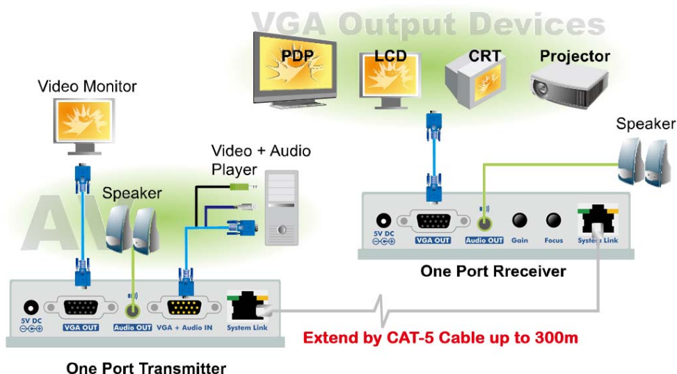
Installation Diagram of Receiver AVE-301R
